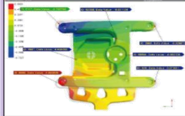
Distortion analysis
