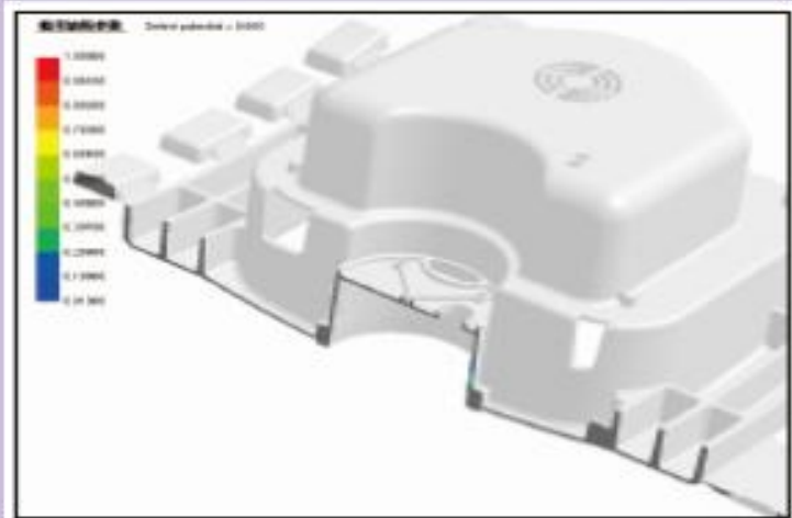
Schrinking defect analysis
